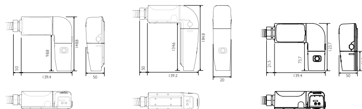
Horizontal 90 Degree Print Head Installation Dimensions
